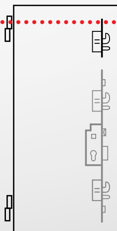
with hooks and anti-lift pin art. 2800054
