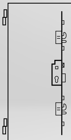
2 hooks 2 anti-lift pins 4 rollers art. 281A201354
