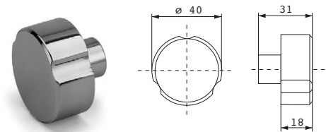
Knob for prearranged cylinder
